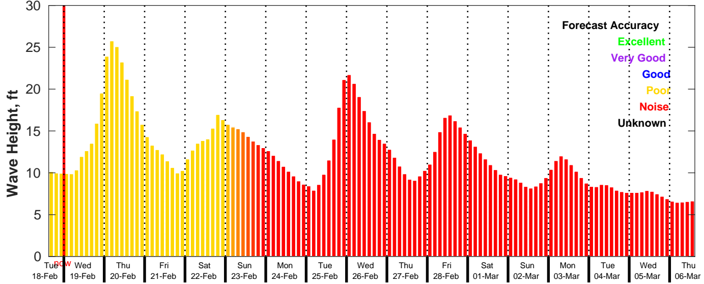
GFS Wave Forecast for NDBC 46246 from 18-Feb-2025 15:00:00 to 06-Mar-2025 15:00:00
