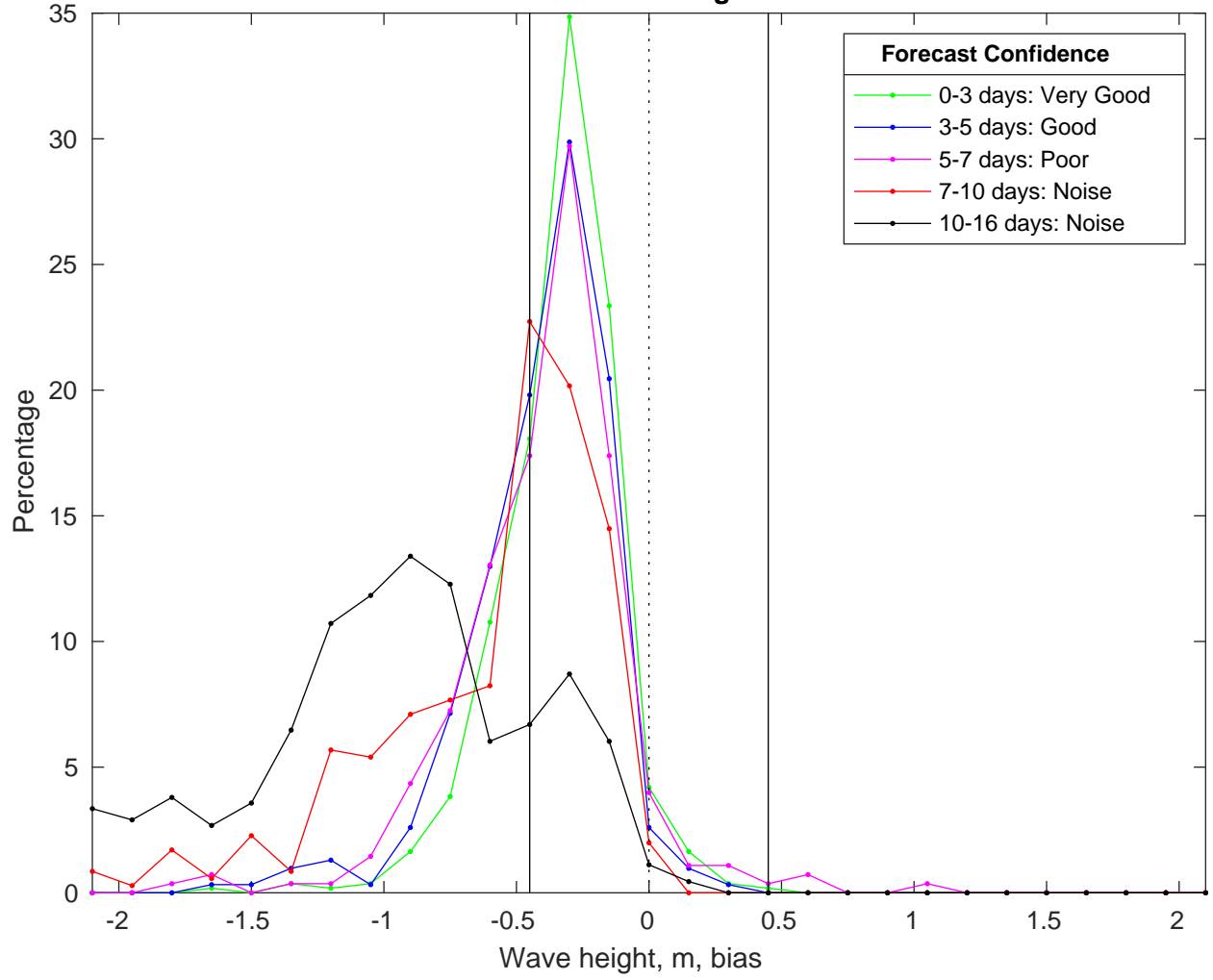
NDBC 51209 vs GFS Waves Bias Histogram: 19-Feb-2025
