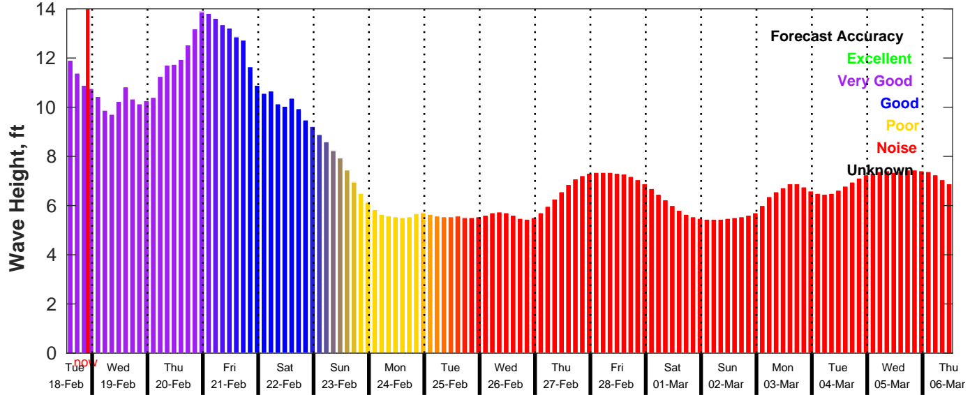
GFS Wave Forecast for NDBC 51209 from 18-Feb-2025 13:00:00 to 06-Mar-2025 13:00:00
