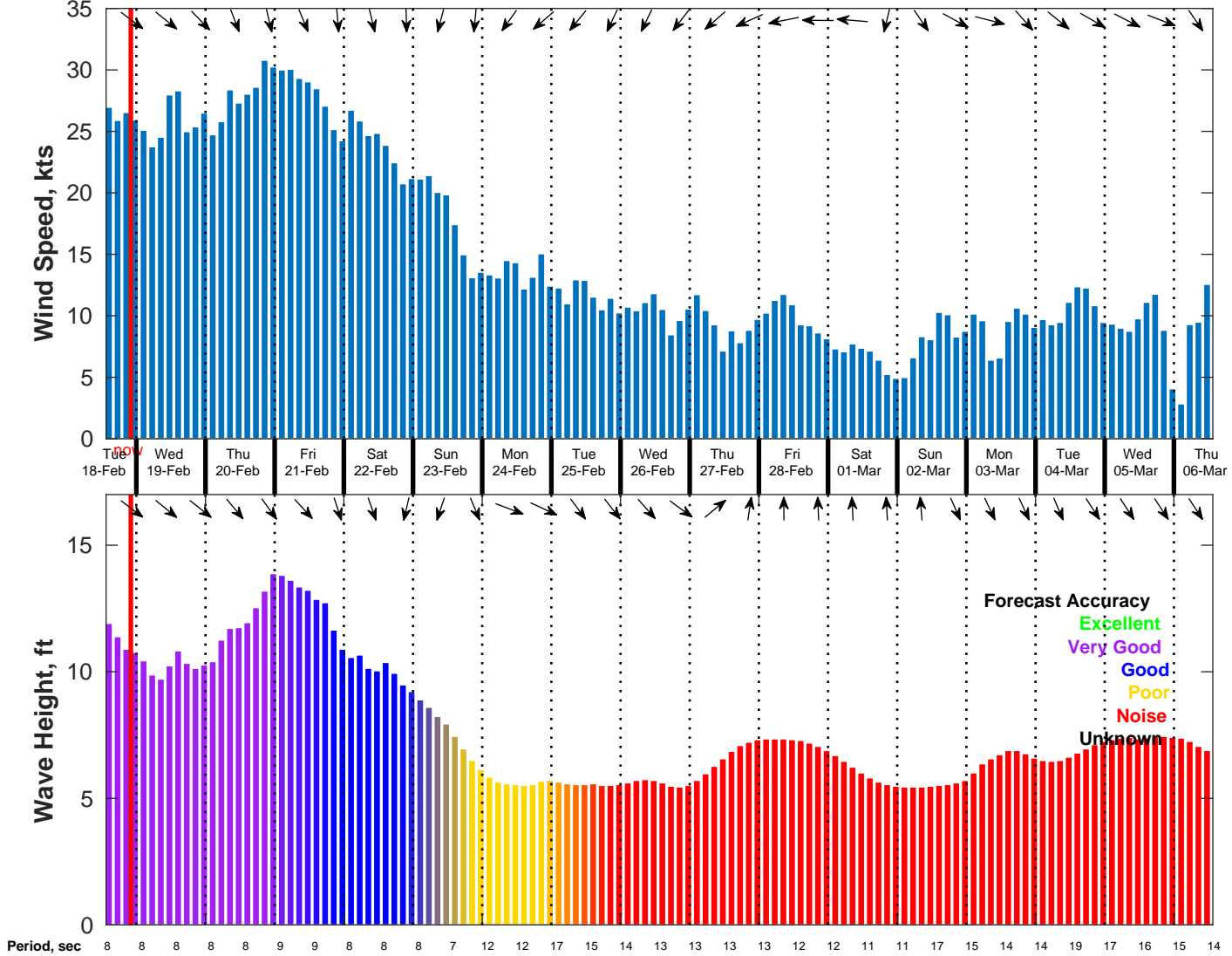
Wind & Wave Forecast for NDBC 51209 from 18-Feb-2025 13:00:00 to 06-Mar-2025 13:00:00
