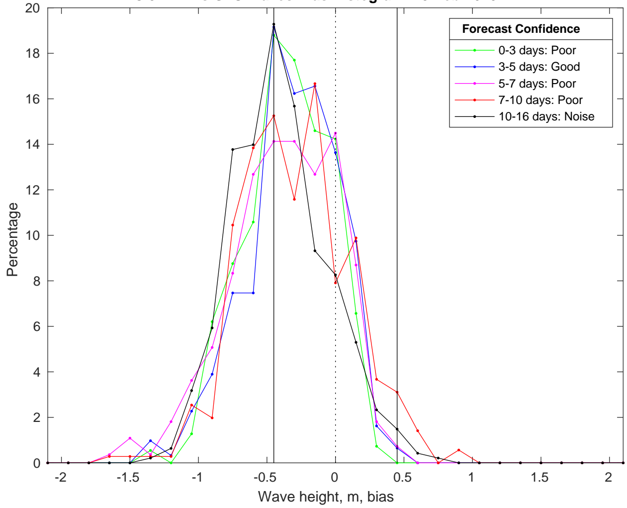
NDBC 52211 vs GFS Waves Bias Histogram: 19-Feb-2025
