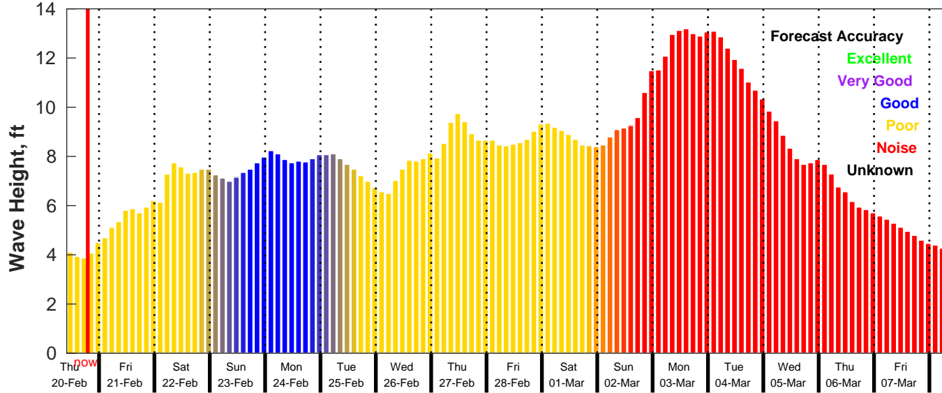
GFS Wave Forecast for NDBC 52211 from 19-Feb-2025 10:00:00 to 07-Mar-2025 10:00:00
