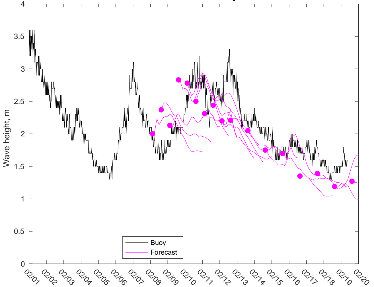
NDBC 52212 vs GFS Waves: 7 to 10 day forecast
