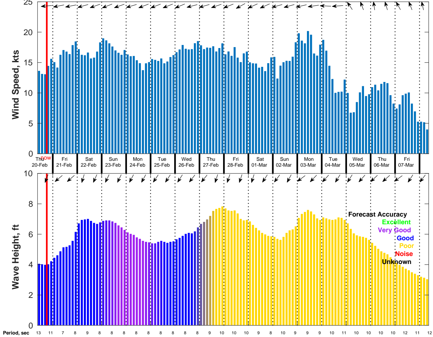
Wind & Wave Forecast for NDBC 52212 from 19-Feb-2025 09:00:00 to 07-Mar-2025 09:00:00
