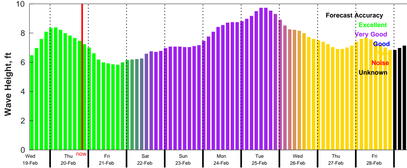
CMEMS Wave Forecast for NDBC 52213 from 18-Feb-2025 11:00:00 to 28-Feb-2025 11:00:00
