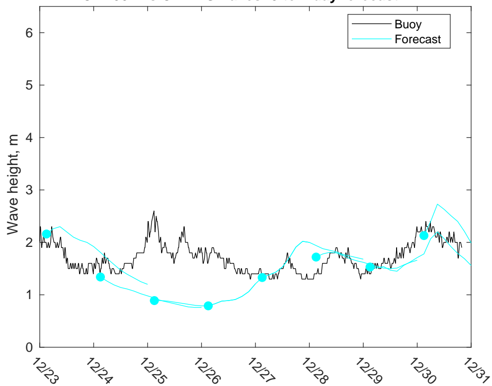
NDBC 41002 vs CMEMSWaves: 5 to 7 day forecast
