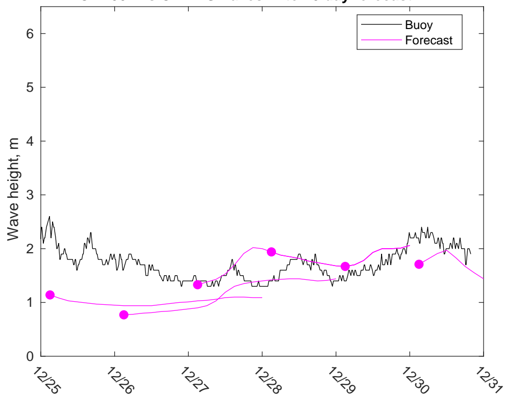
NDBC 41002 vs CMEMSWaves: 7 to 10 day forecast
