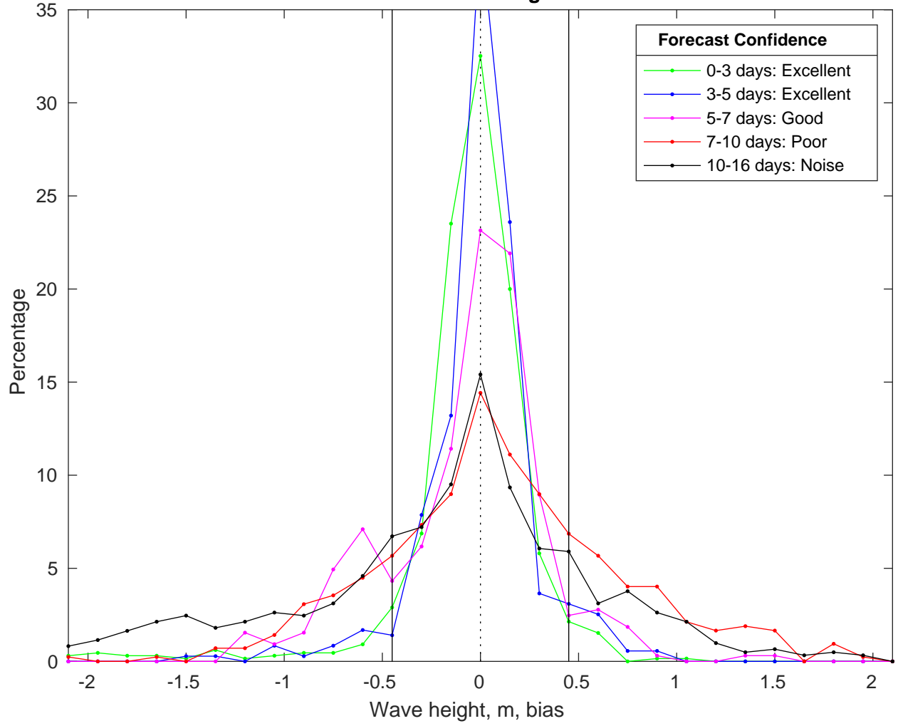
NDBC 41004 vs GFS Waves Bias Histogram: 20-Feb-2025
