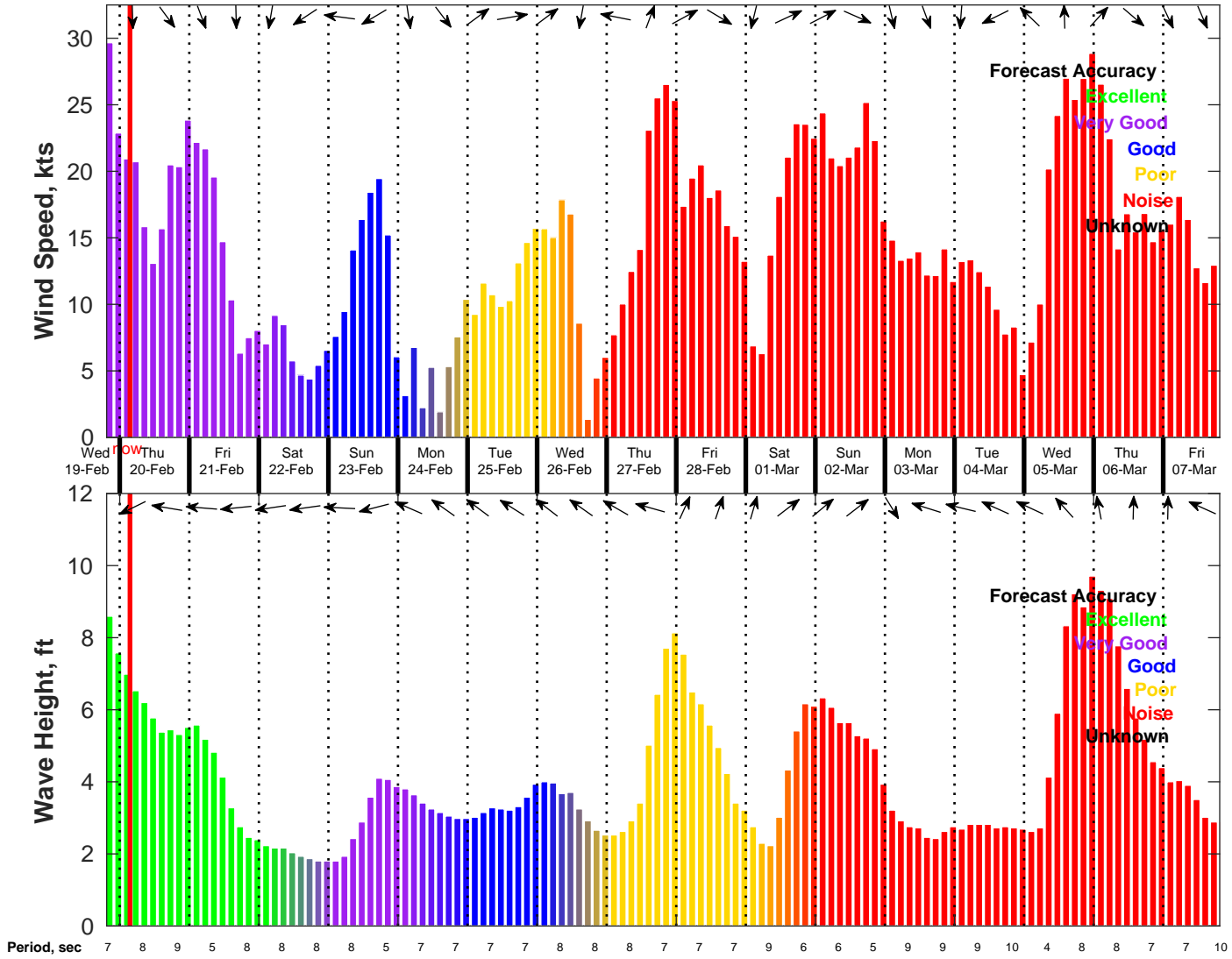
Wind & Wave Forecast for NDBC 41013 from 19-Feb-2025 19:00:00 to 07-Mar-2025 19:00:00
