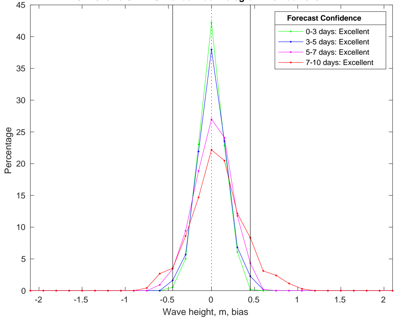
NDBC 41040 vs CMEMS Waves Bias Histogram: 20-Feb-2025
