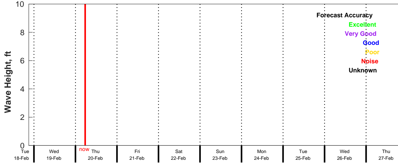
CMEMS Wave Forecast for NDBC 41040 from 18-Feb-2025 21:00:00 to 27-Feb-2025 21:00:00
