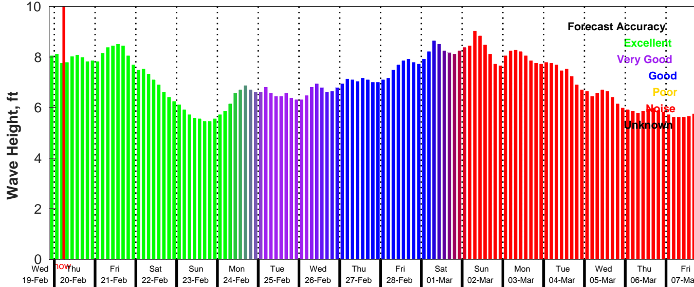
GFS Wave Forecast for NDBC 41040 from 19-Feb-2025 21:00:00 to 07-Mar-2025 21:00:00
