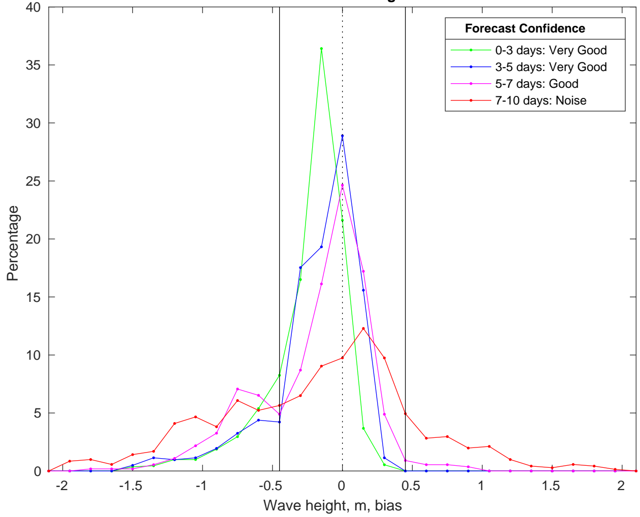
NDBC 42019 vs CMEMS Waves Bias Histogram: 20-Feb-2025
