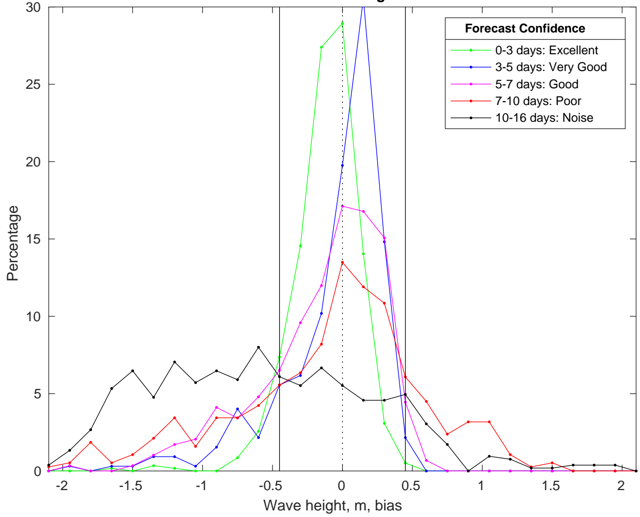
NDBC 42019 vs GFS Waves Bias Histogram: 20-Feb-2025
