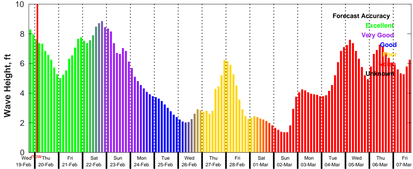
GFS Wave Forecast for NDBC 42019 from 19-Feb-2025 18:00:00 to 07-Mar-2025 18:00:00
