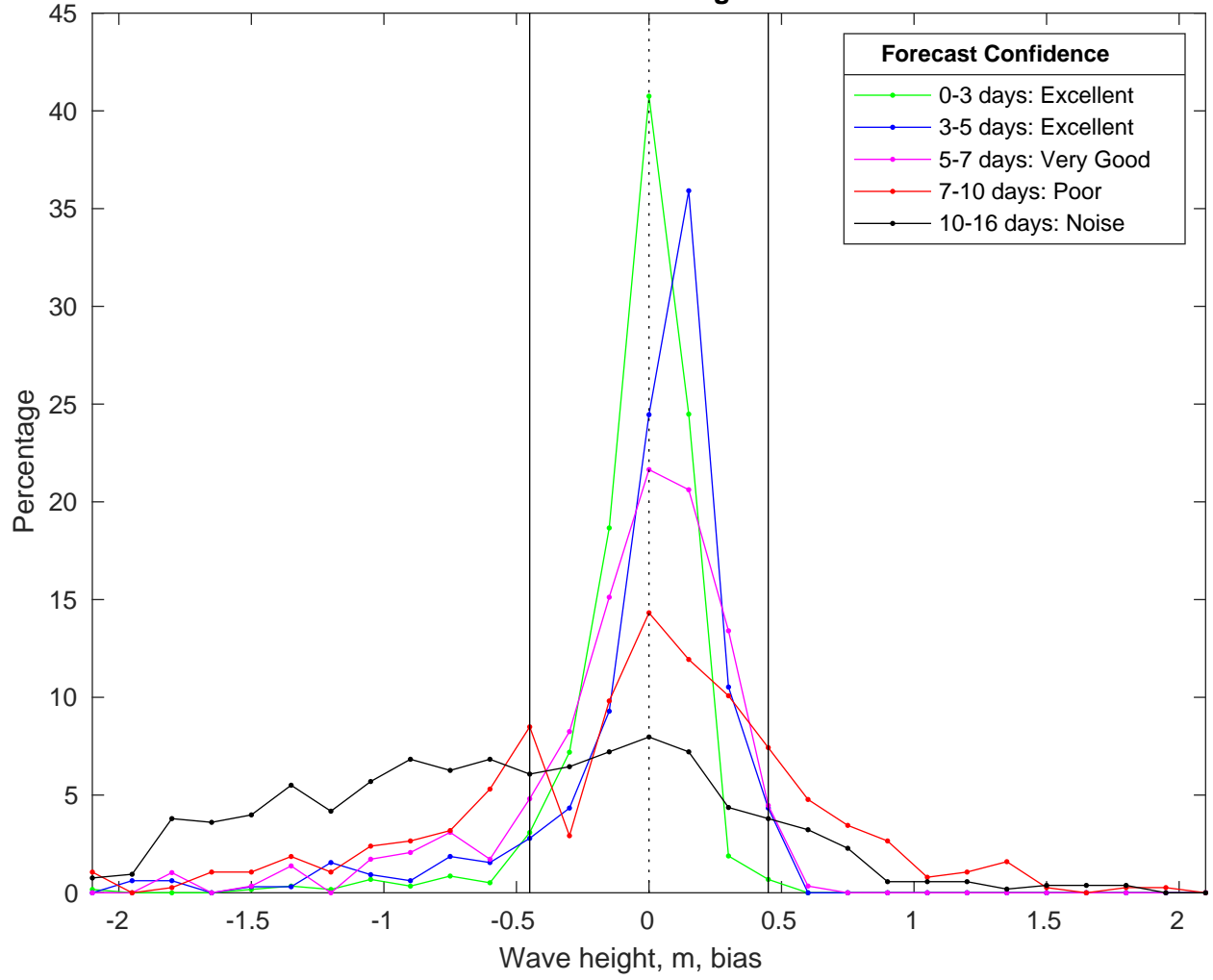
NDBC 42020 vs GFS Waves Bias Histogram: 20-Feb-2025
