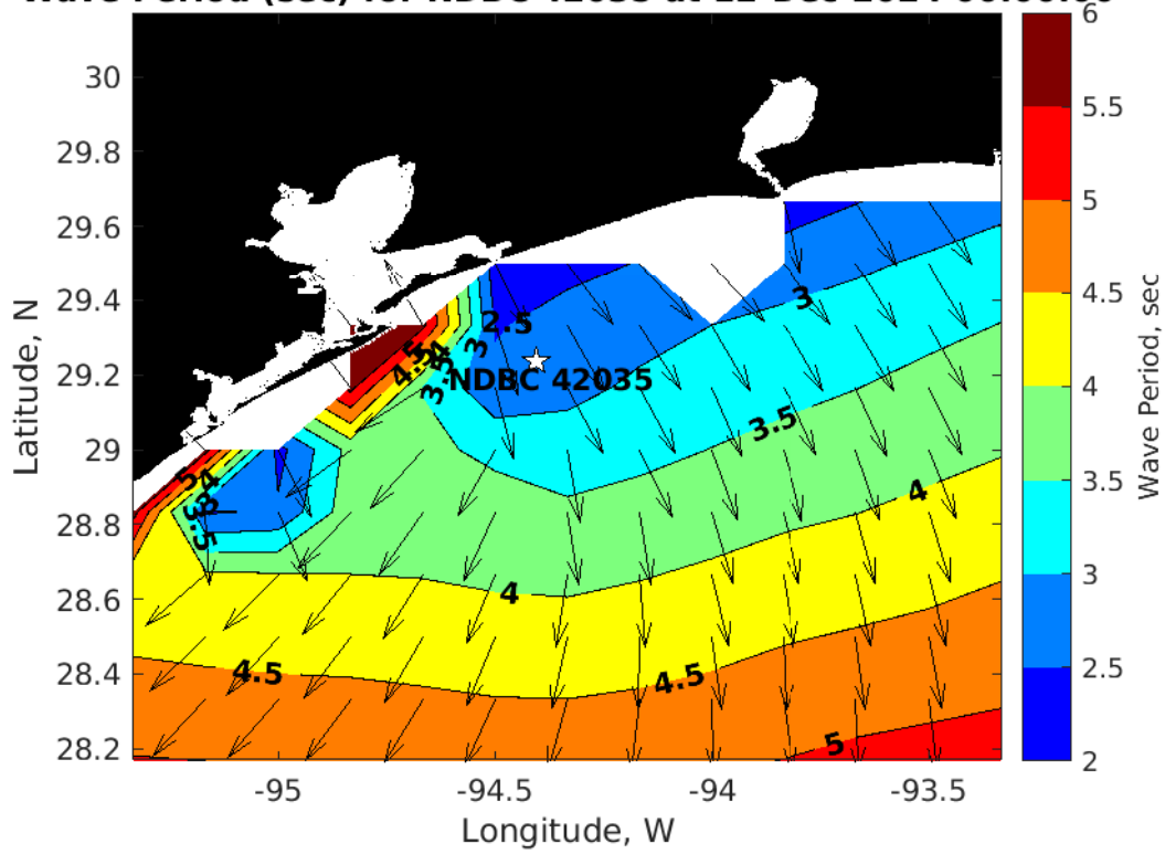
Wave Period (sec) for NDBC 42035 at 12-Dec-2024 00:00:00
