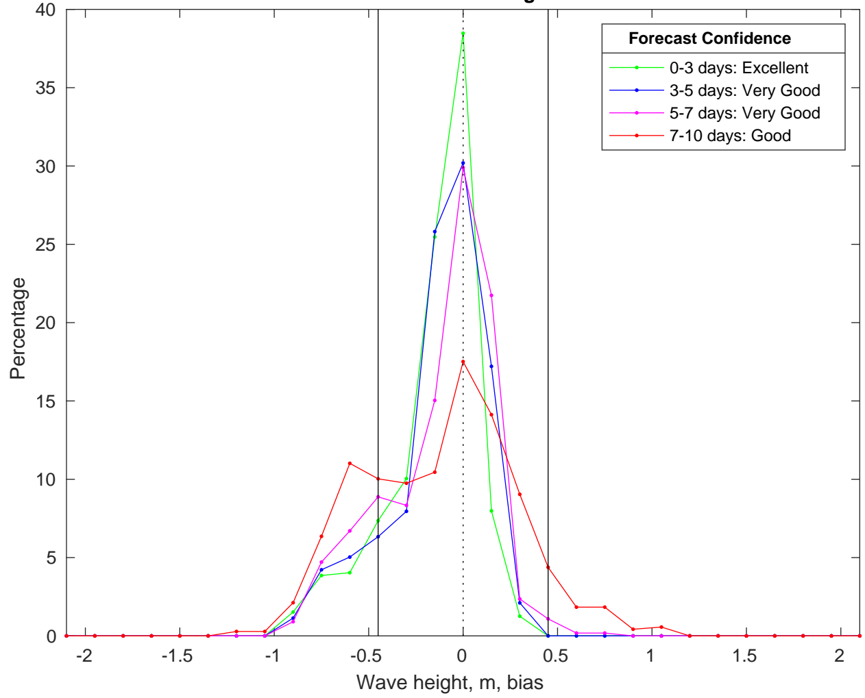
NDBC 42035 vs CMEMS Waves Bias Histogram: 20-Feb-2025
