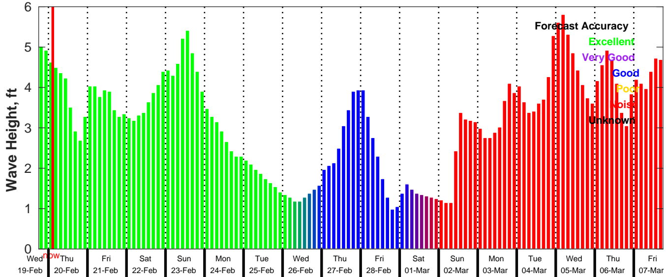
GFS Wave Forecast for NDBC 42035 from 19-Feb-2025 18:00:00 to 07-Mar-2025 18:00:00
