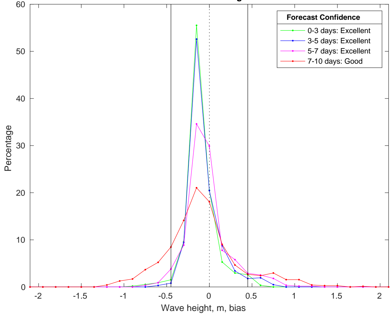
NDBC 42036 vs CMEMS Waves Bias Histogram: 20-Feb-2025
