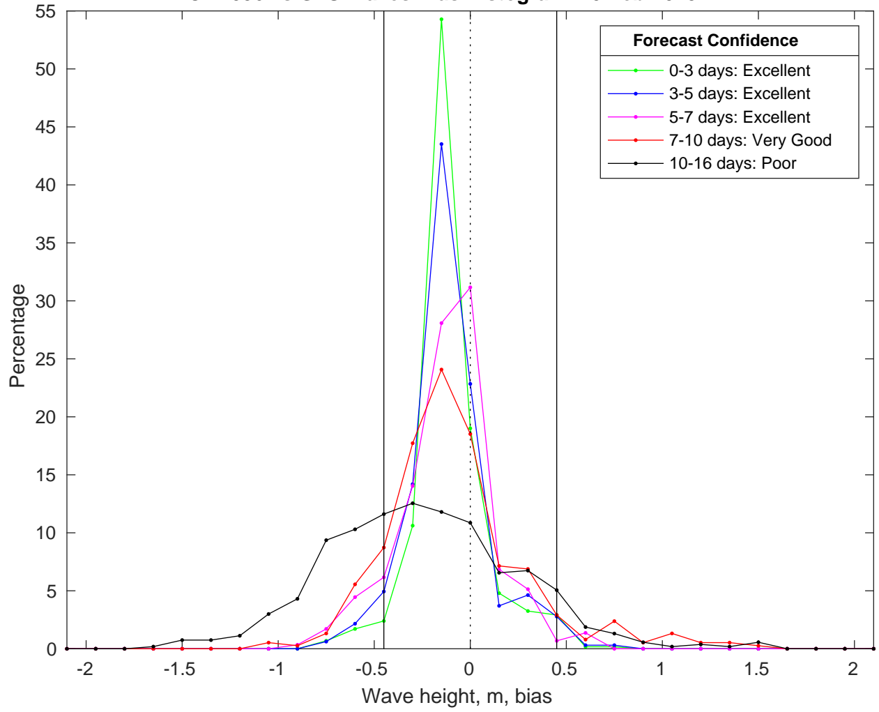
NDBC 42036 vs GFS Waves Bias Histogram: 20-Feb-2025
