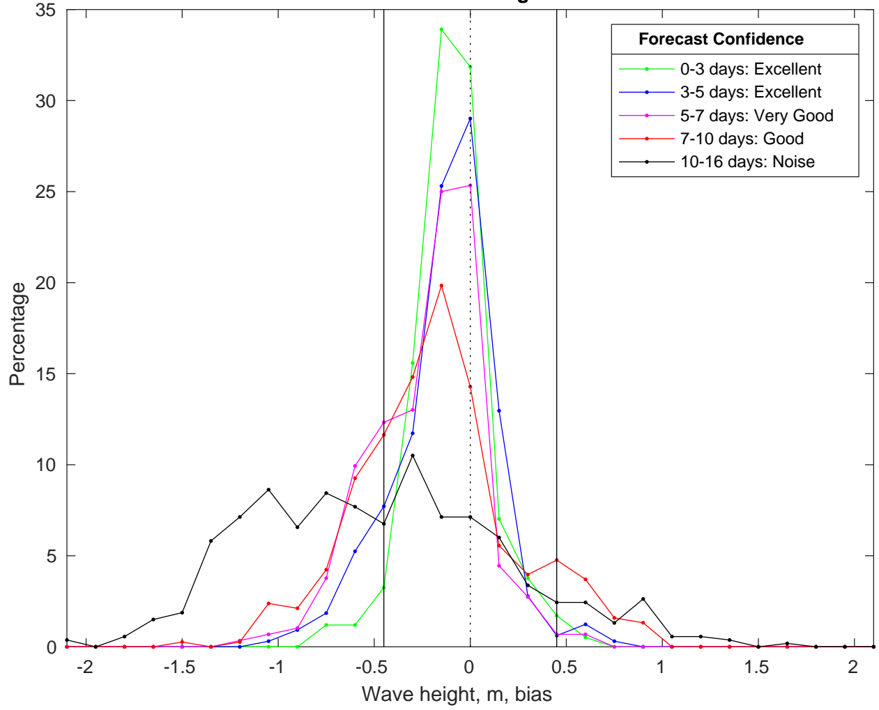
NDBC 42040 vs GFS Waves Bias Histogram: 20-Feb-2025
