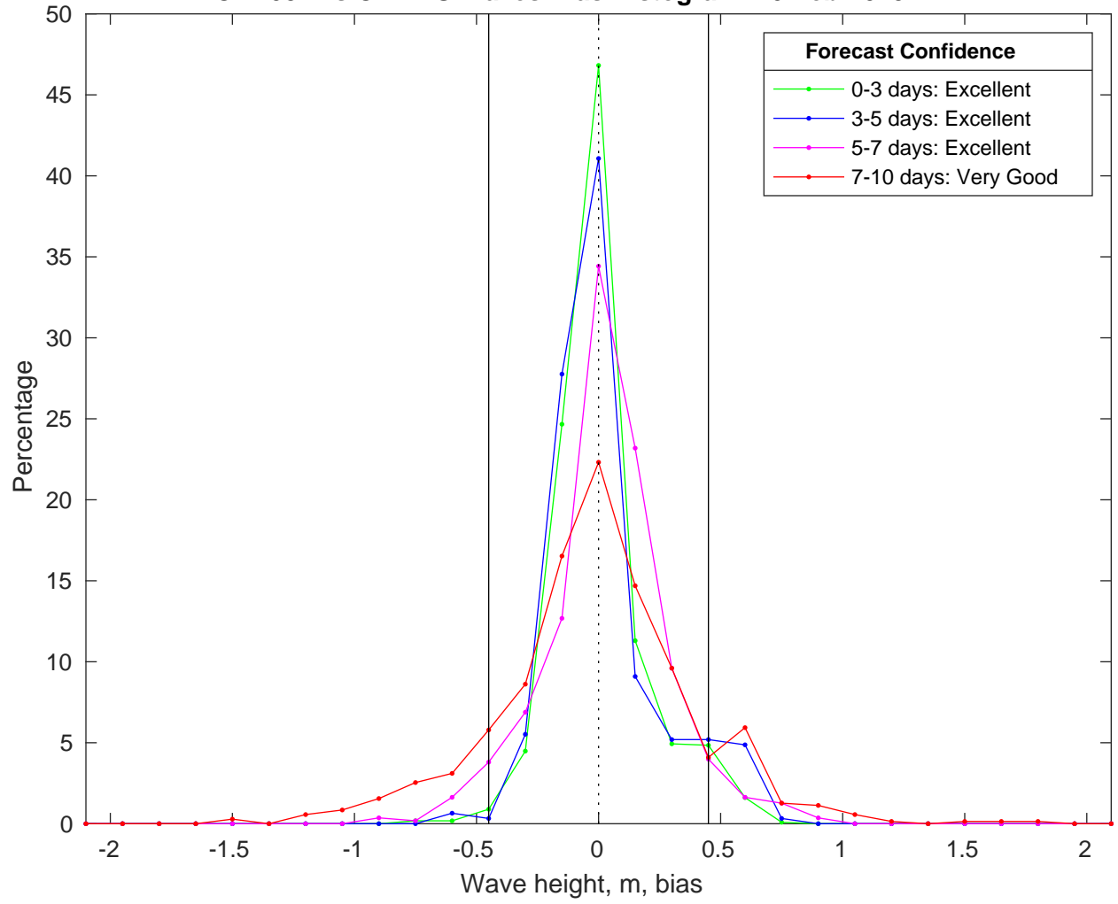
NDBC 42084 vs CMEMS Waves Bias Histogram: 20-Feb-2025
