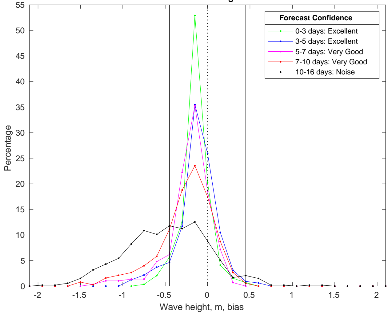
NDBC 42084 vs GFS Waves Bias Histogram: 20-Feb-2025
