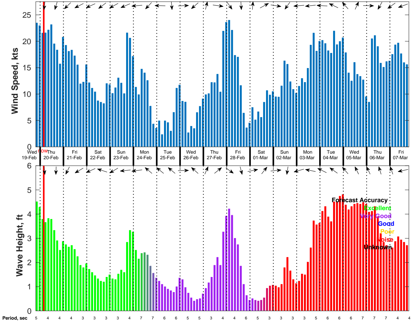
Wind & Wave Forecast for NDBC 42084 from 19-Feb-2025 19:00:00 to 07-Mar-2025 19:00:00
