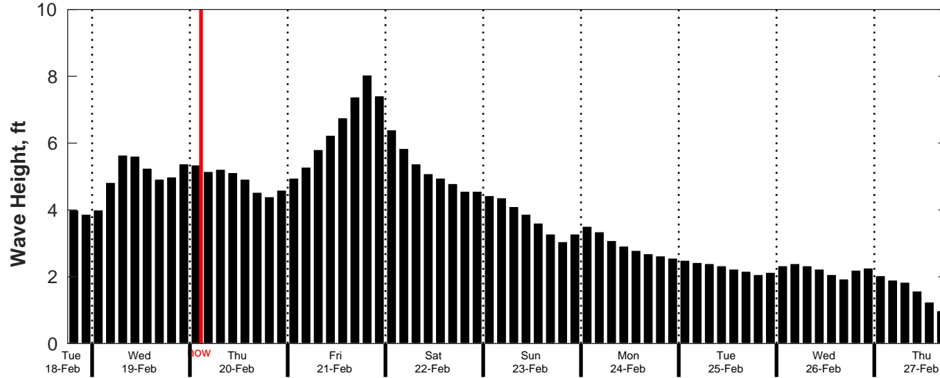
CMEMS Wave Forecast for NDBC 42092 from 18-Feb-2025 18:00:00 to 27-Feb-2025 18:00:00
