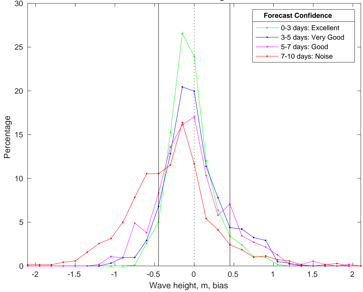
NDBC 46011 vs CMEMS Waves Bias Histogram: 20-Feb-2025
