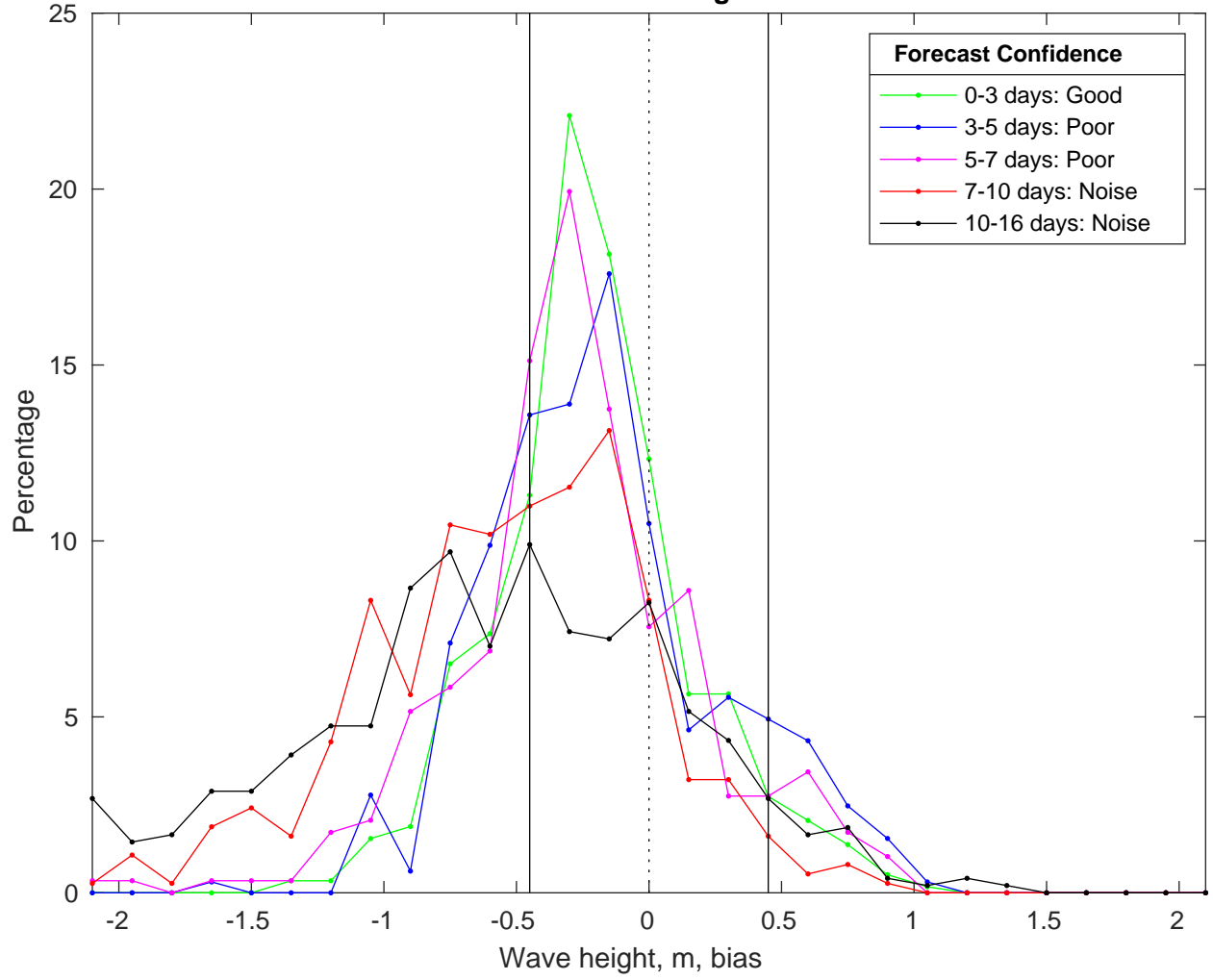
NDBC 46011 vs GFS Waves Bias Histogram: 20-Feb-2025
