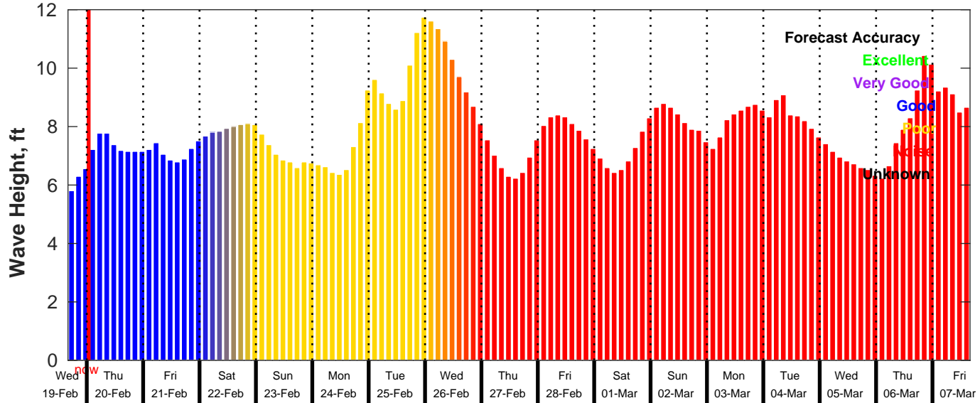
GFS Wave Forecast for NDBC 46011 from 19-Feb-2025 16:00:00 to 07-Mar-2025 16:00:00
