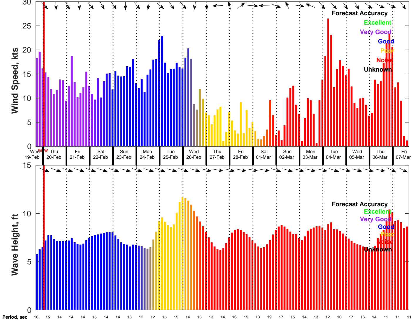
Wind & Wave Forecast for NDBC 46011 from 19-Feb-2025 16:00:00 to 07-Mar-2025 16:00:00
