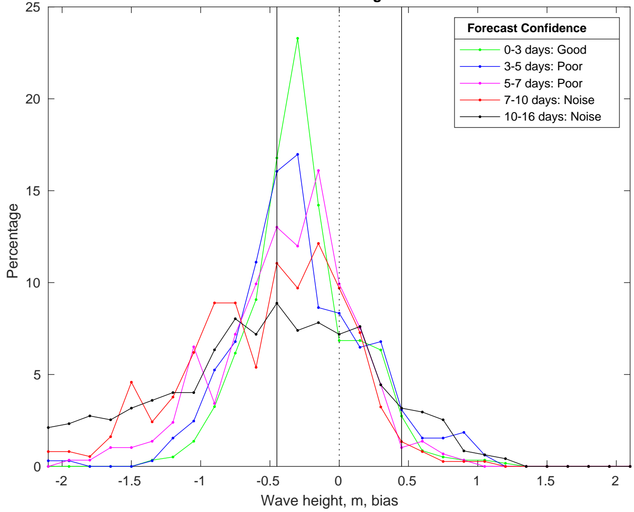
NDBC 46028 vs GFS Waves Bias Histogram: 20-Feb-2025
