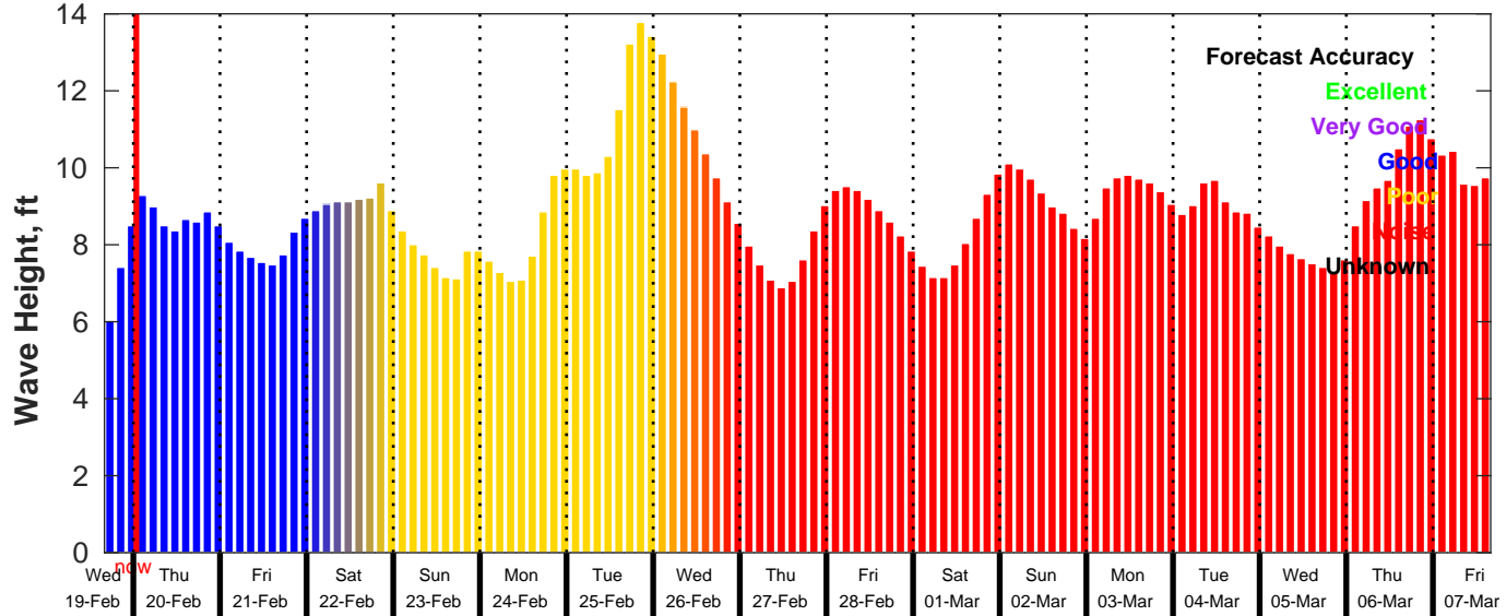
GFS Wave Forecast for NDBC 46028 from 19-Feb-2025 16:00:00 to 07-Mar-2025 16:00:00
