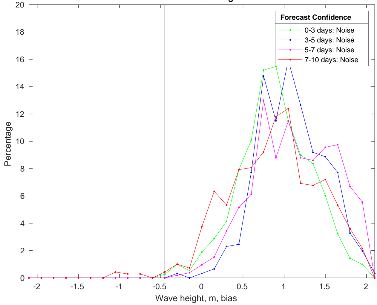
NDBC 46053 vs CMEMS Waves Bias Histogram: 20-Feb-2025
