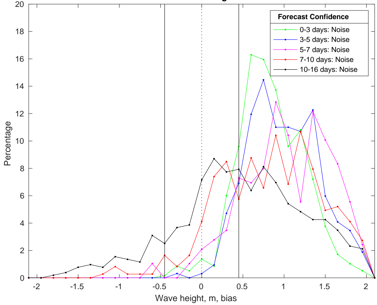
NDBC 46053 vs GFS Waves Bias Histogram: 20-Feb-2025
