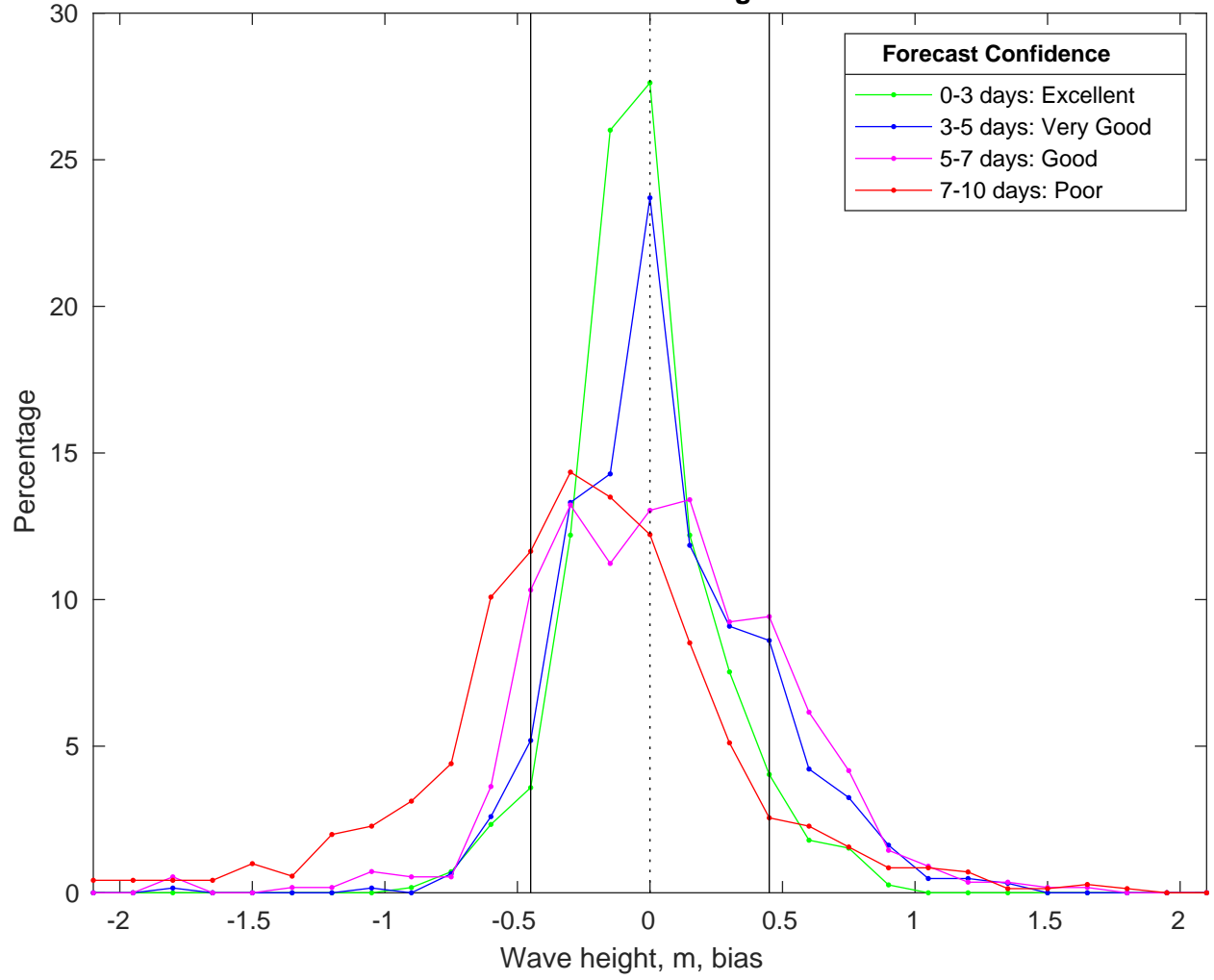
NDBC 46054 vs CMEMS Waves Bias Histogram: 20-Feb-2025
