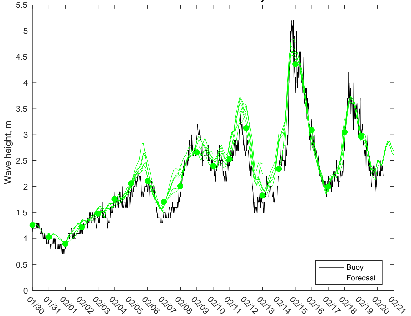
NDBC 46069 vs CMEMS Waves: 0 to 3 day forecast
