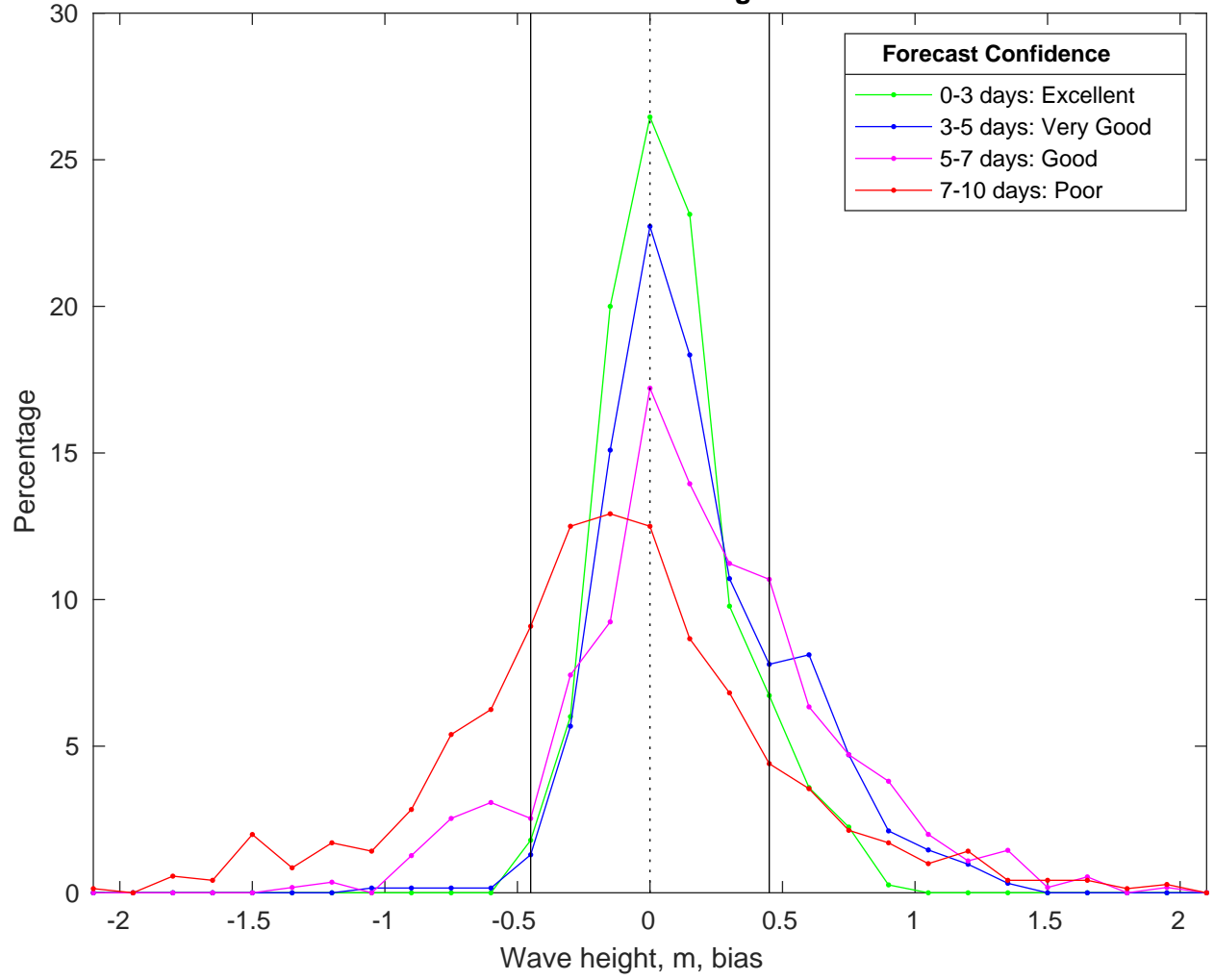
NDBC 46069 vs CMEMS Waves Bias Histogram: 20-Feb-2025
