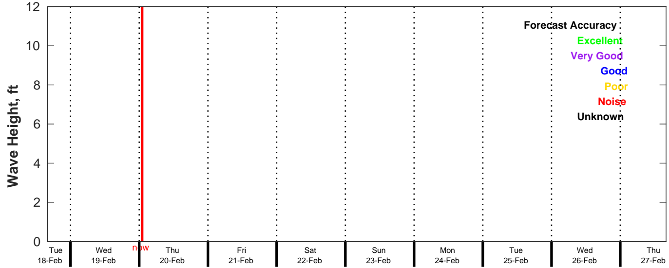
CMEMS Wave Forecast for NDBC 46069 from 18-Feb-2025 16:00:00 to 27-Feb-2025 16:00:00
