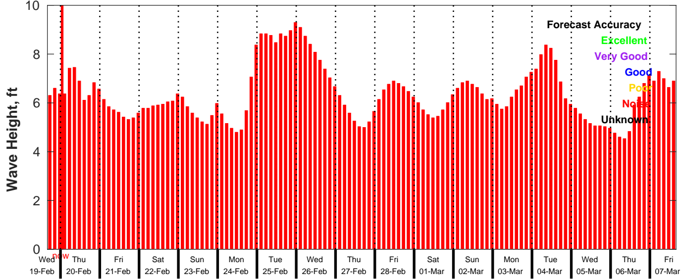
GFS Wave Forecast for NDBC 46069 from 19-Feb-2025 16:00:00 to 07-Mar-2025 16:00:00
