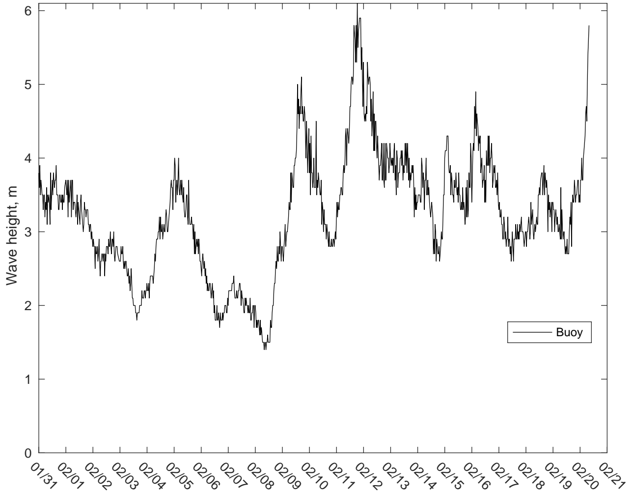
NDBC 46246 vs CMEMS Waves: 10 to 16 day forecast
