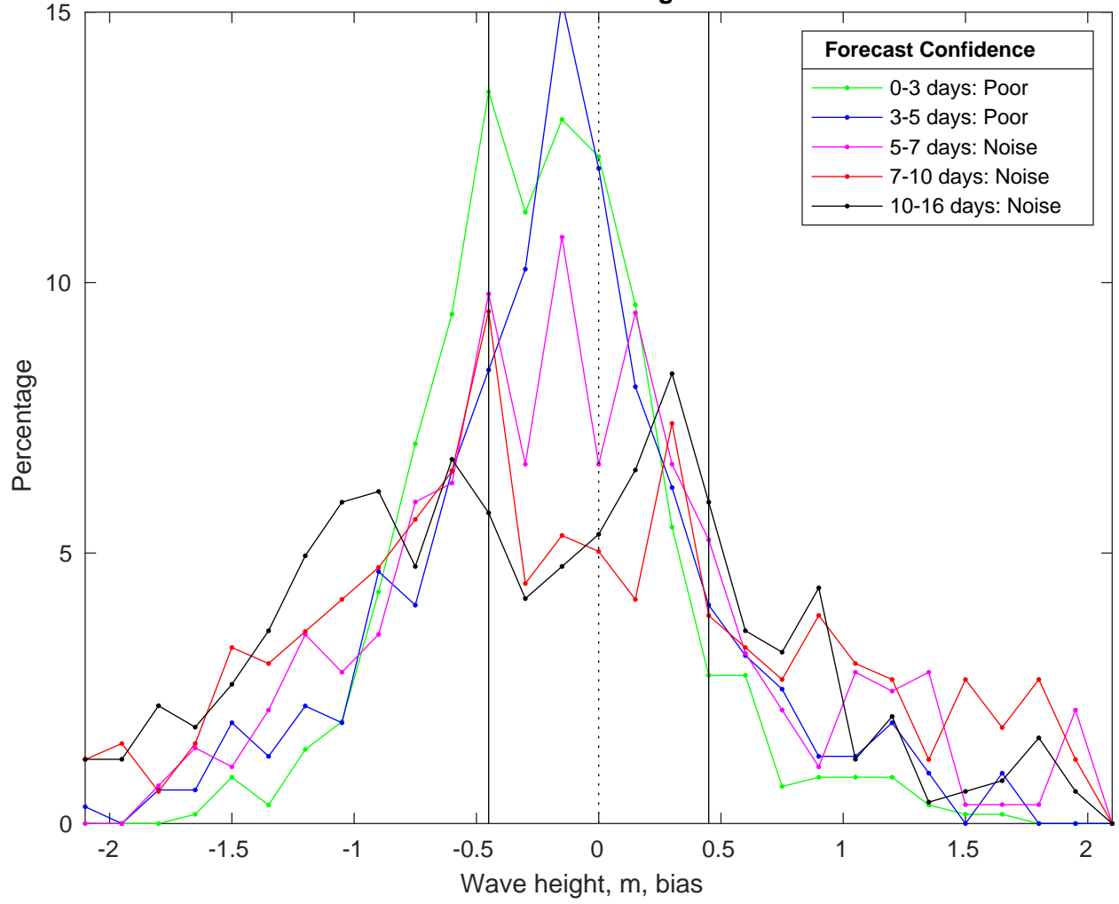
NDBC 46246 vs GFS Waves Bias Histogram: 20-Feb-2025
