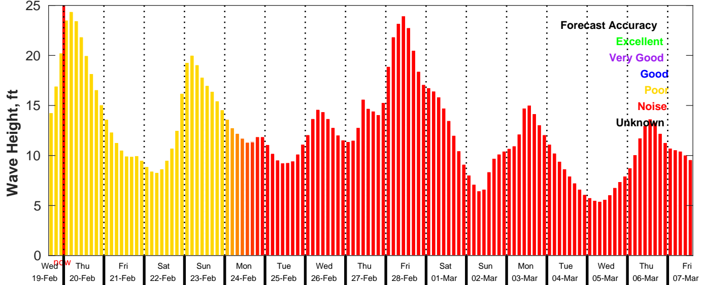
GFS Wave Forecast for NDBC 46246 from 19-Feb-2025 15:00:00 to 07-Mar-2025 15:00:00
