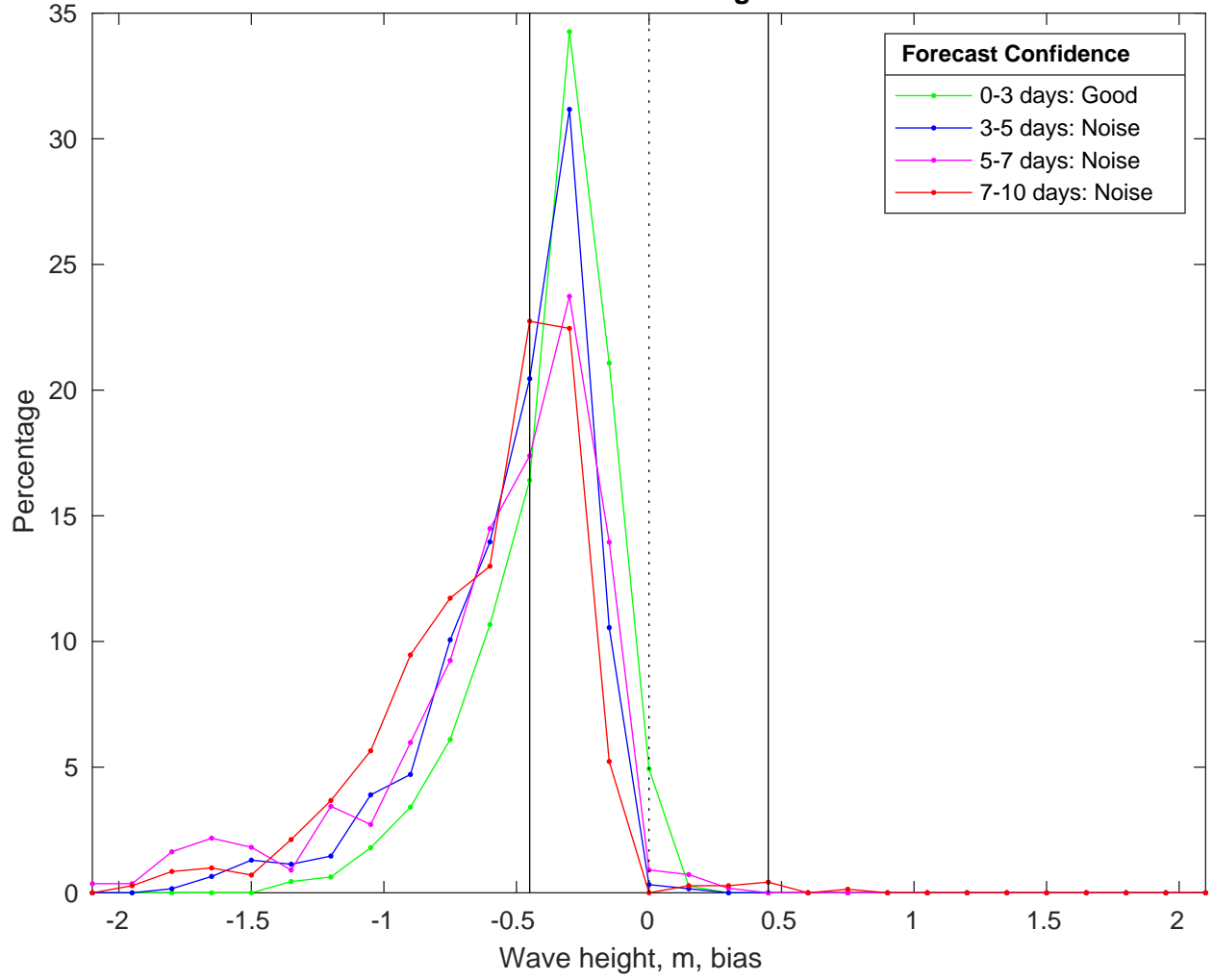
NDBC 51209 vs CMEMS Waves Bias Histogram: 20-Feb-2025
