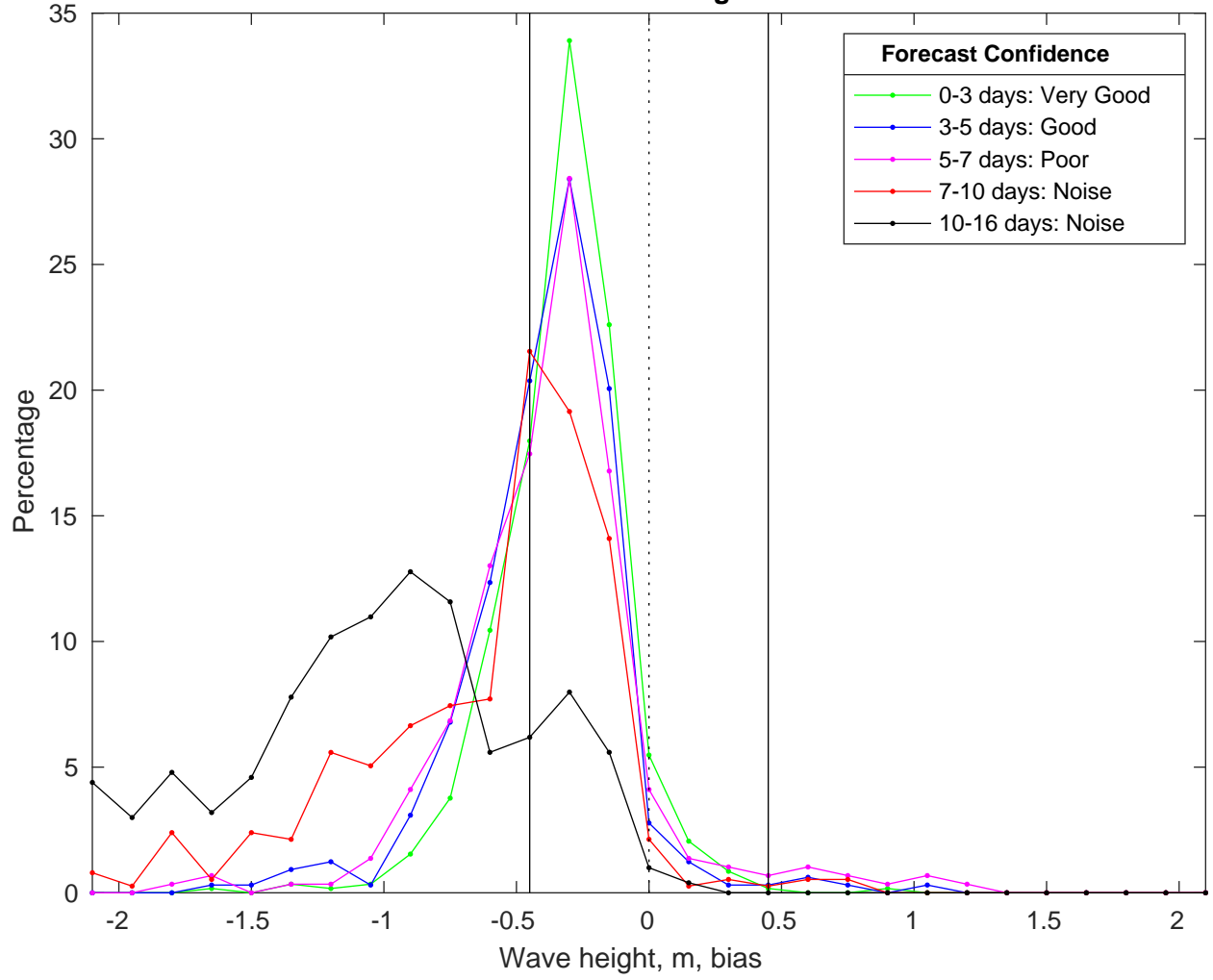
NDBC 51209 vs GFS Waves Bias Histogram: 20-Feb-2025
