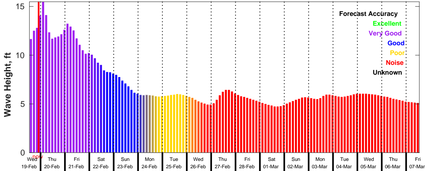
GFS Wave Forecast for NDBC 51209 from 19-Feb-2025 13:00:00 to 07-Mar-2025 13:00:00
