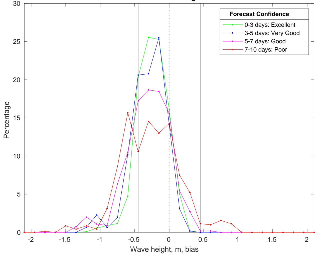
NDBC 52211 vs CMEMS Waves Bias Histogram: 20-Feb-2025
